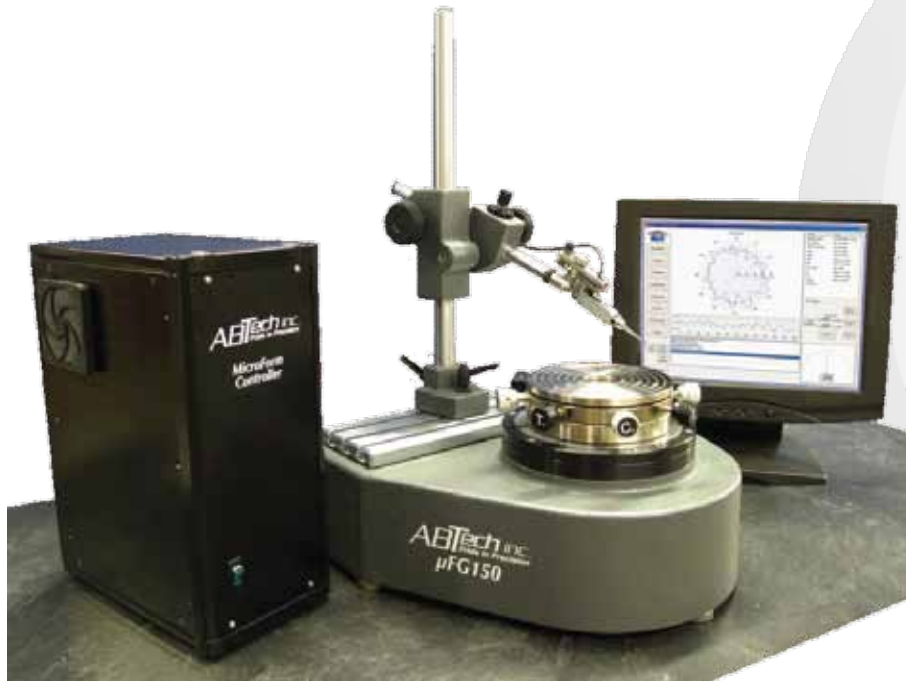
MicroForm™ Gage Model μFG150
